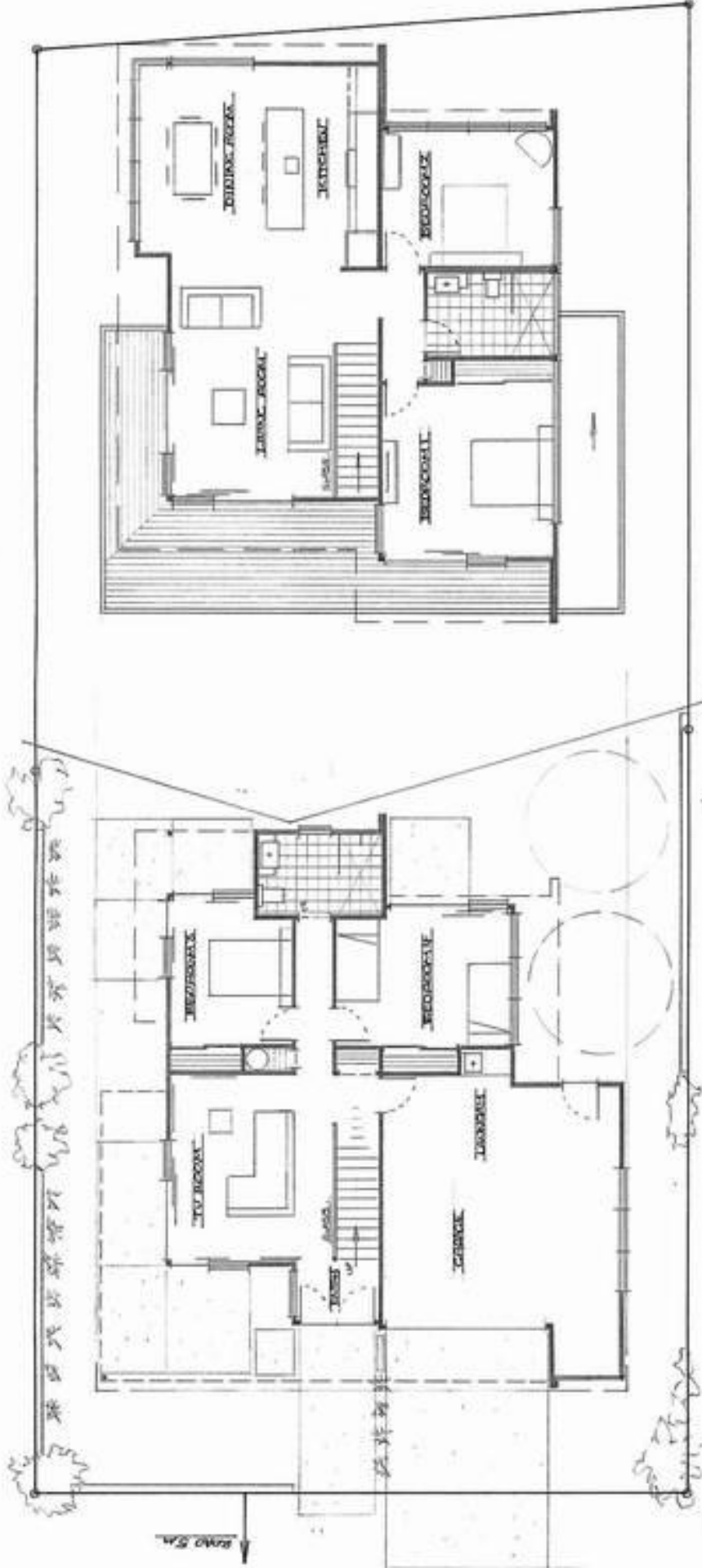
SITE PLAN -S.A.M. 11/80-
